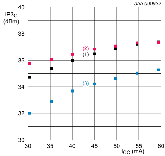
V_{CC} = 5\text{ V} ; P_i = -15\text{ dBm} per tone; T_{amb} = 25\text{ }^\circ\text{C} . (1) f = 2000\text{ MHz} (2) f = 2500\text{ MHz} (3) f = 3000\text{ MHz}
